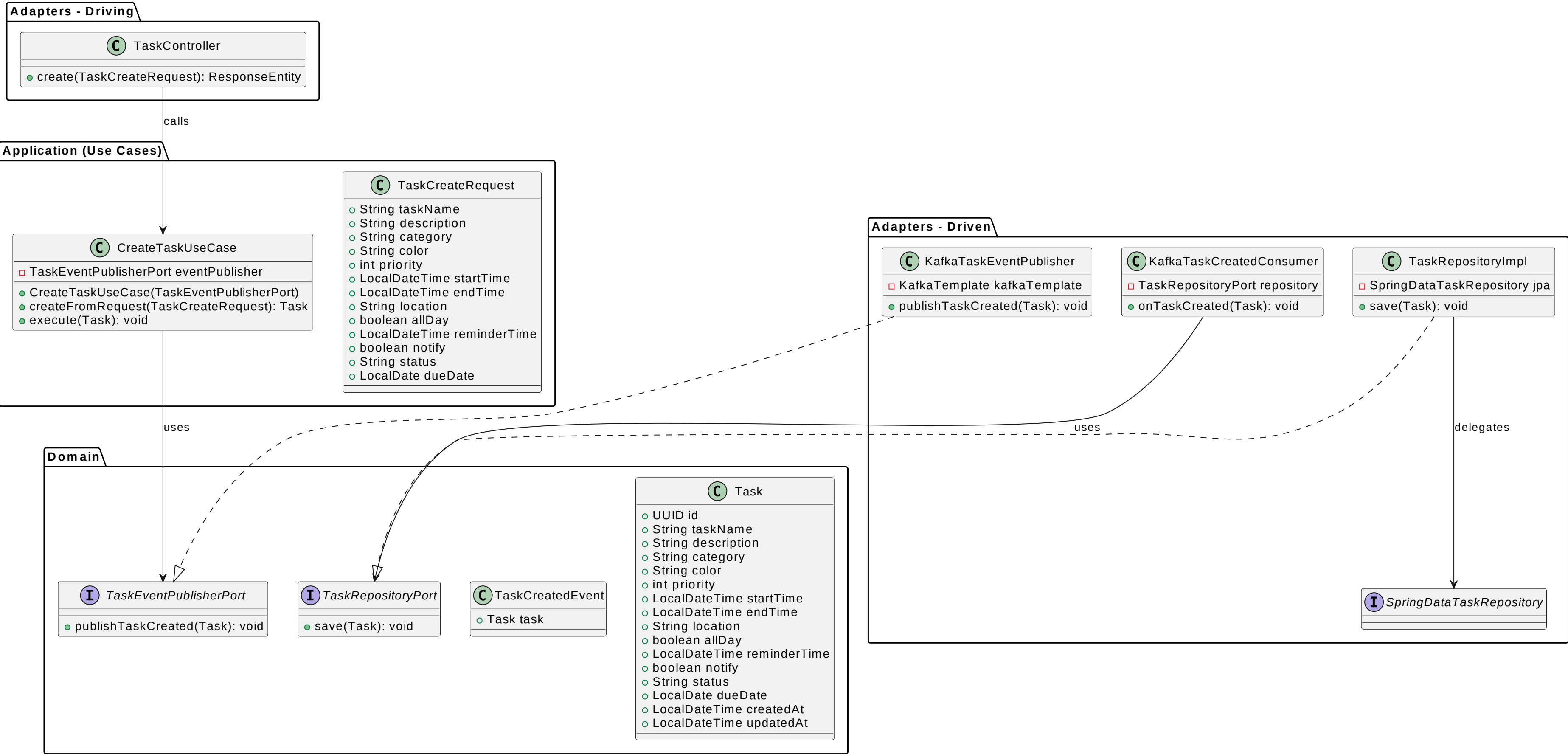
Class Diagram - Clean Architecture (POST /tasks/create)
